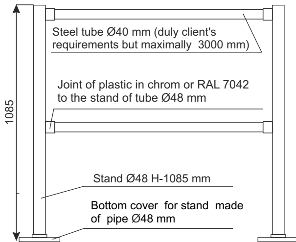
ROOM PARTITION H-1085 mm:
