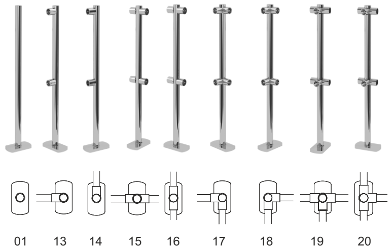
COMPLETE STAND CONFIGURATIONS H-1085 (stand with bottom cover and joints):
